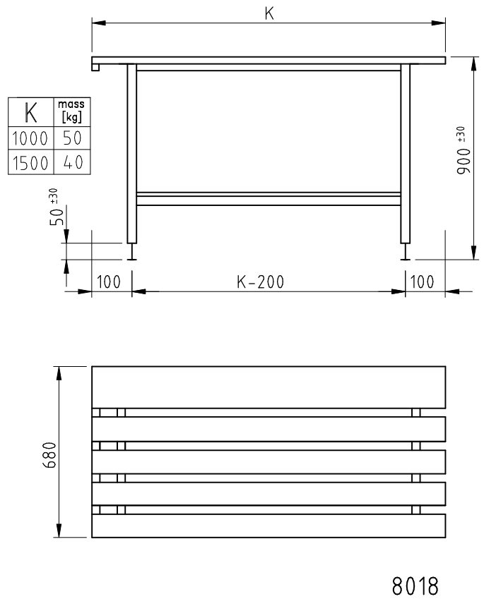
Ironing-table
