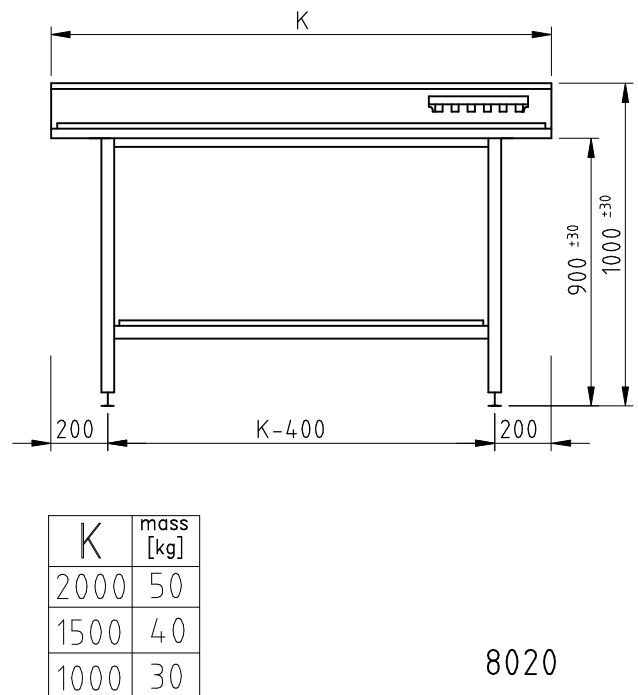
Ironing-table
